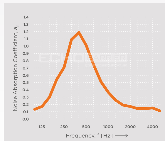
NOISE ABSORPTION
